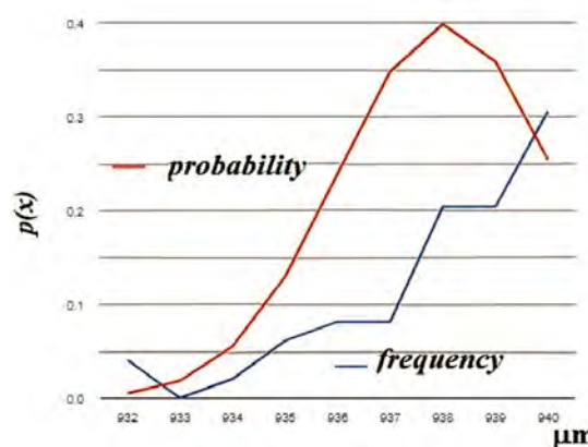
Fig. 9. Empirical frequency polygon and probability for the normal law of distribution of the data array
