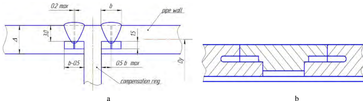
Fig. 5. Working form of assembly and welding of pipes: a – through the compensation ring; b – when working out the modes on planar samples
