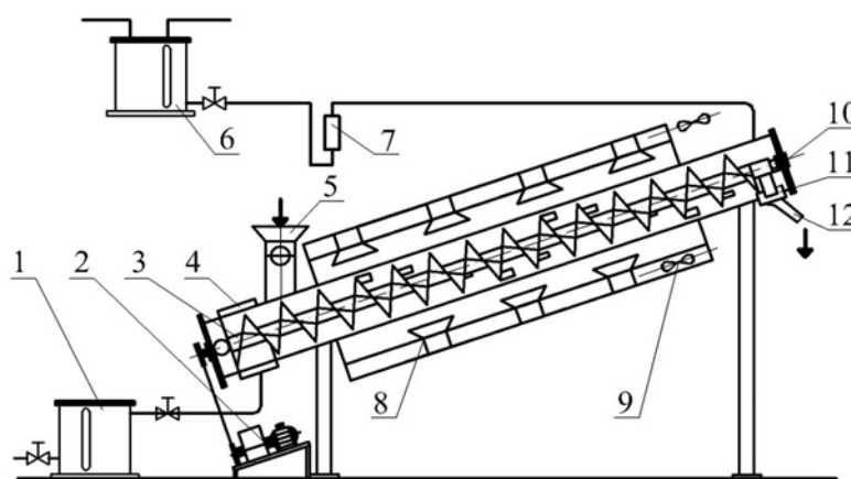
The screw microwave extractor design: 1 – the extract collector, 2 – the drive, 3 – the screw, 4 – the sieve belt, 5 – a loading bunker, 6 – the container with extractant, 7 – a rotameter, 8 – the magnetrons with horn antenna, 9 – a fan, 10 – a stopcock, 11 – a kickoff blade, 12 – a tray
