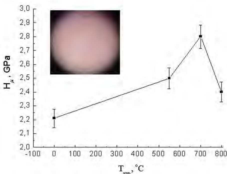
Fig. 6. Dependence on temperature microhardness ZnMnO arson in an oxygen atmosphere (insert - image of an indent)
