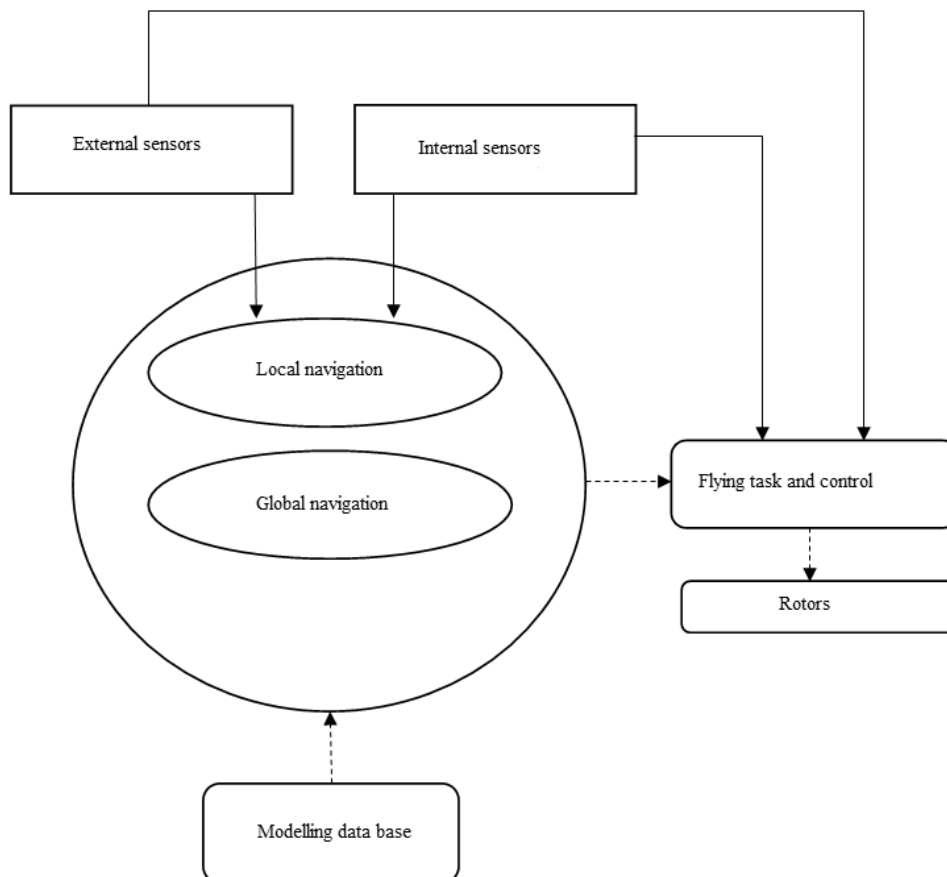
Diagram of the remote-piloted vehicle positioning in the absence of GNSS signals based on the target onboard equipment
