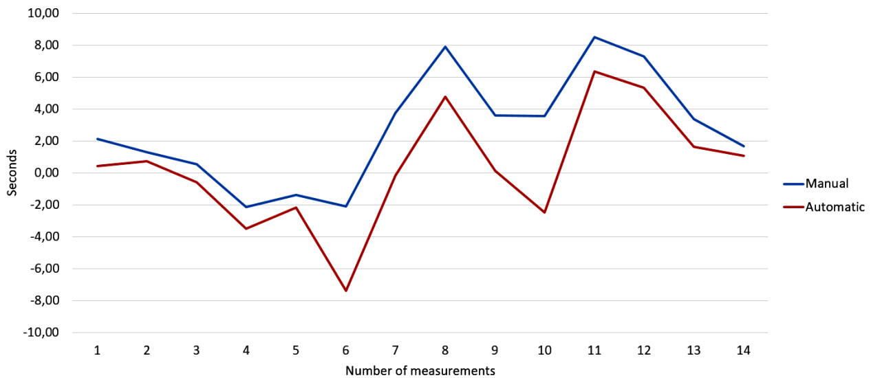
Fig. 8. Comparison of the dt2 values difference between manual and automated measurements
