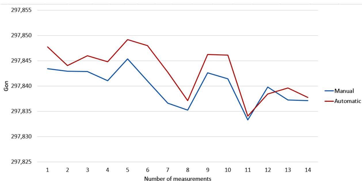
Fig. 6. Comparison of the Azimuth values between manual and automated measurements (gon)
