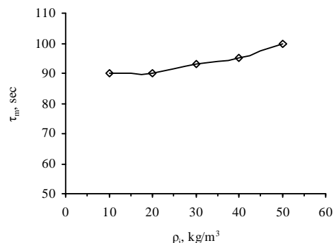
Fig. 7. Influence of apparent density of the sample on time of achieving FPS maximum density in butanol at 363 K
