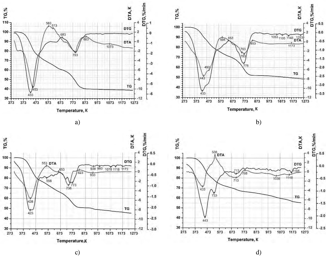
Fig. 2. Thermogravimetric analysis of xerogel powders of the CaO-ZrO 2 -Nb 2 O 5 -SiO 2 system: ZN-1 (a); ZN-3 (b); ZN-10 (c) and ZN-40 (d)
