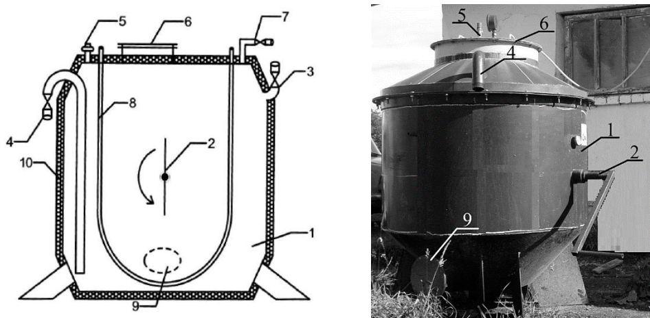
Fig. 1. Bioreactor scheme:
