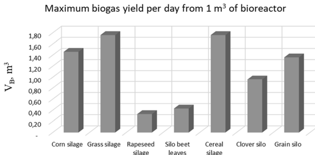
Fig. 2. The maximum daily value of biogas output from agricultural biomass, V_B , m 3
