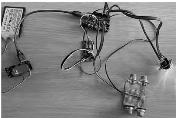
Fig. 2. Components of the meat control and identification system
