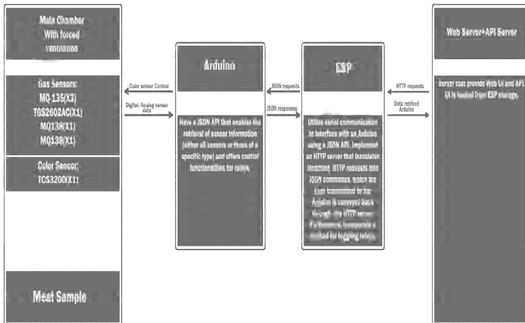
Fig. 1. Block scheme of the meat control and identification system
