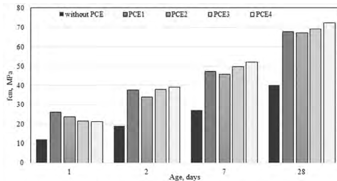
Fig. 2. Compressive strength of concretes based on CEM II/A-LL 42.5 R with PCE
