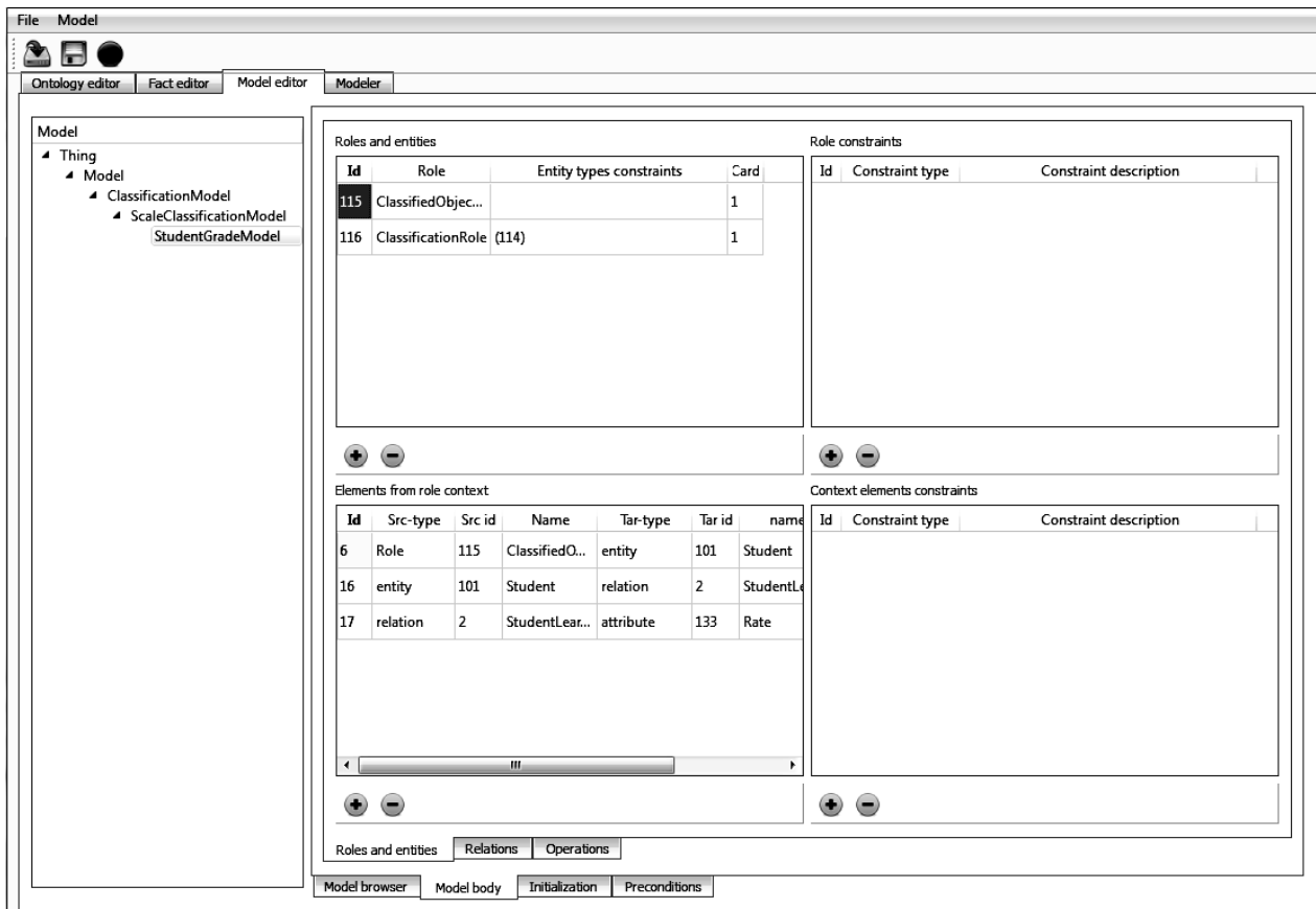
Fig. 5. Model editor
