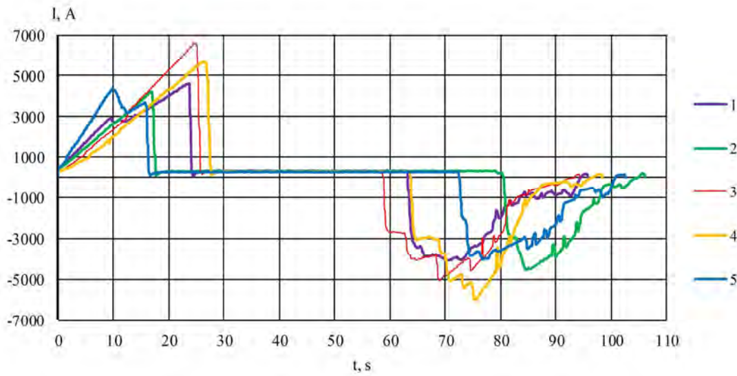
Fig. 7. Oscillograms of current, when an underground train is driven by different train drivers on a specific track section.
