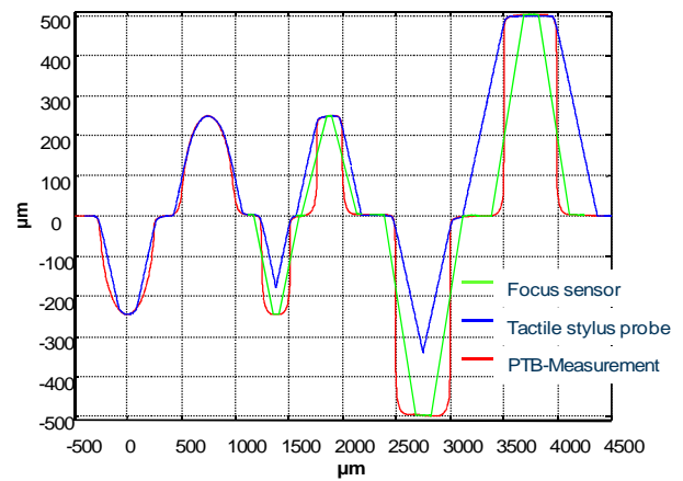
Fig. 8. Comparison of microcontour measurements
